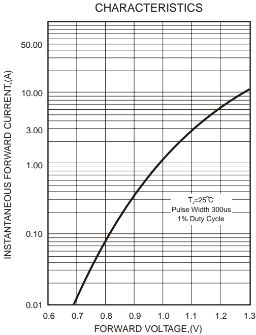
FIG.1-TYPICAL FORWARD CHARACTERISTICS
