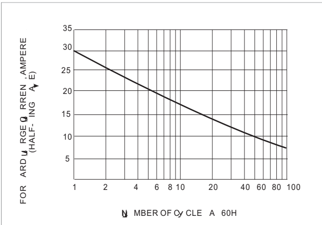
FIGURE 4. MAXIMUM NON-REPELIBLE FORWARD CURRENT
