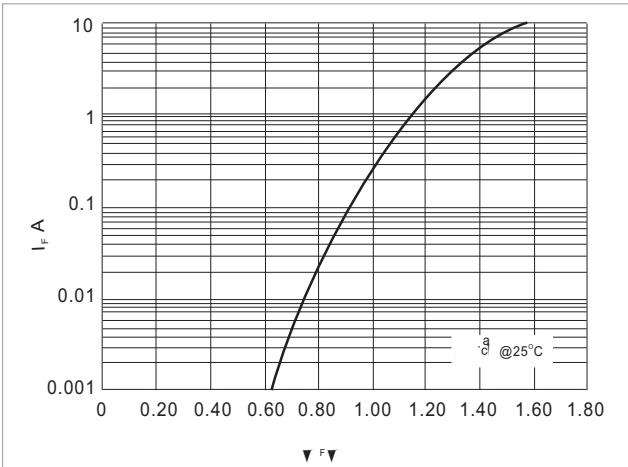
FIGURE 1. TYPICAL FORWARD CHARACTERISTIC
